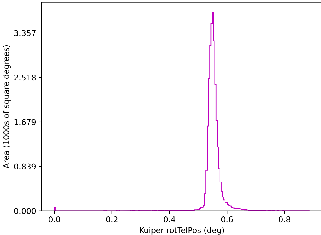
too_elab_r256_d3_giz_v3.4_10yrs z: Kuiper rotTelPos
