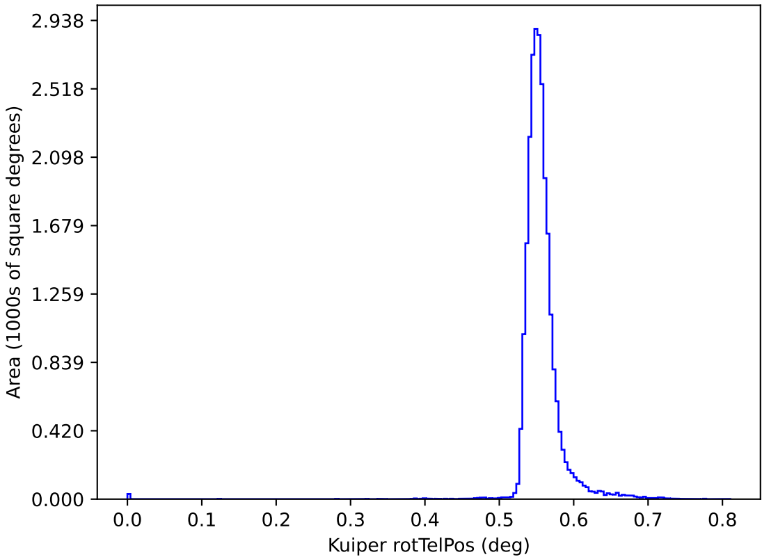
too_elab_r256_d3_giz_v3.4_10yrs y: Kuiper rotTelPos
