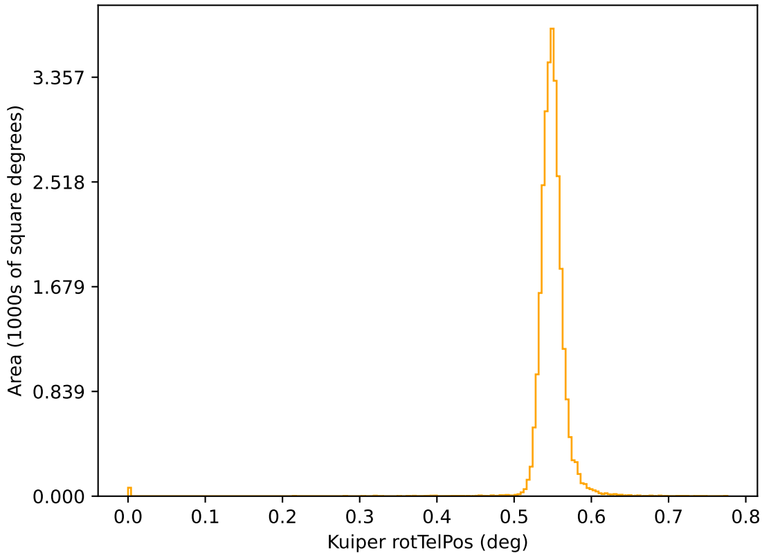
too_elab_r256_d3_giz_v3.4_10yrs r: Kuiper rotTelPos
