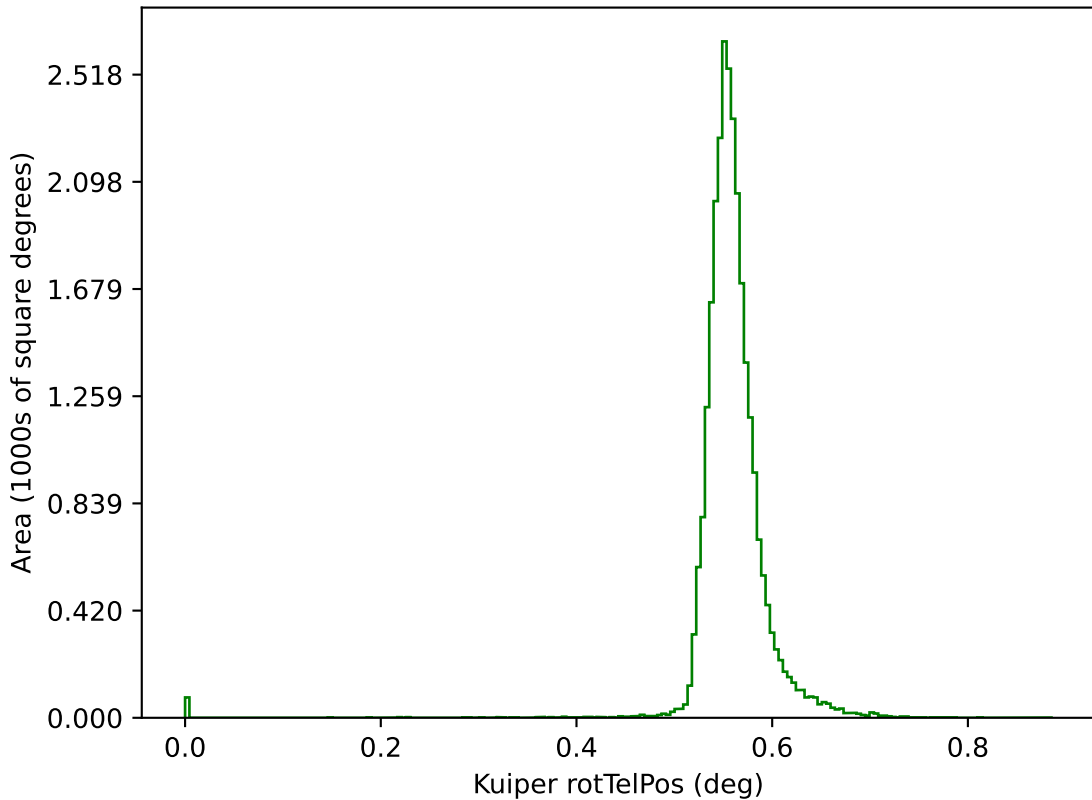
too_elab_r256_d3_giz_v3.4_10yrs g: Kuiper rotTelPos
