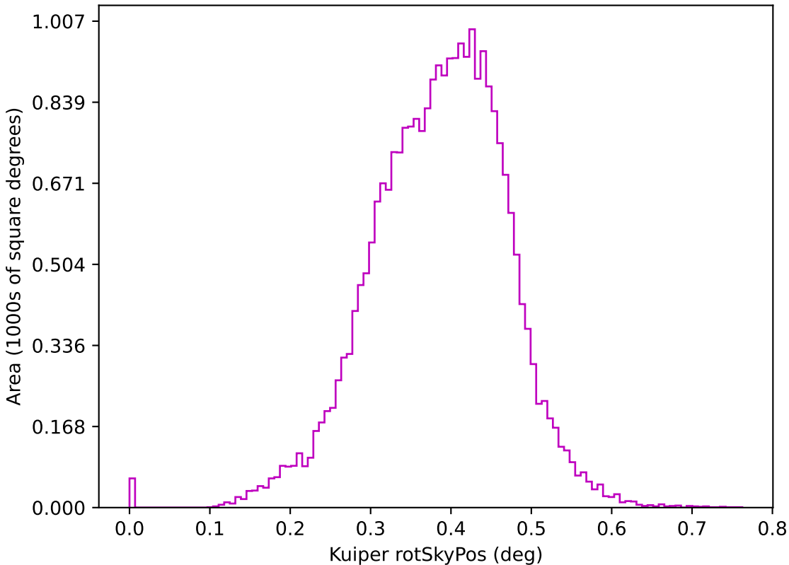
too_elab_r256_d3_giz_v3.4_10yrs z: Kuiper rotSkyPos
