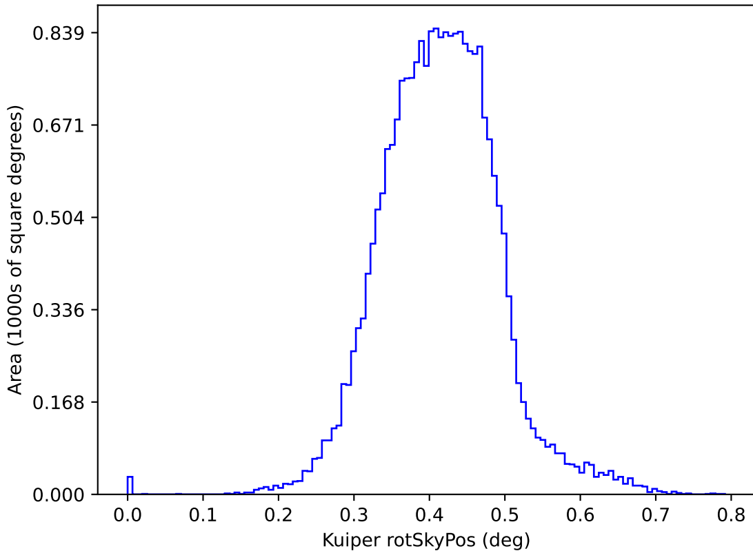
too_elab_r256_d3_giz_v3.4_10yrs y: Kuiper rotSkyPos
