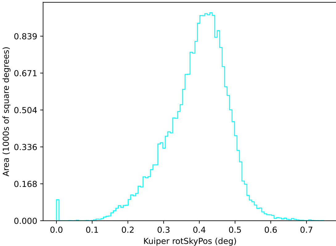
too_elab_r256_d3_giz_v3.4_10yrs u: Kuiper rotSkyPos
