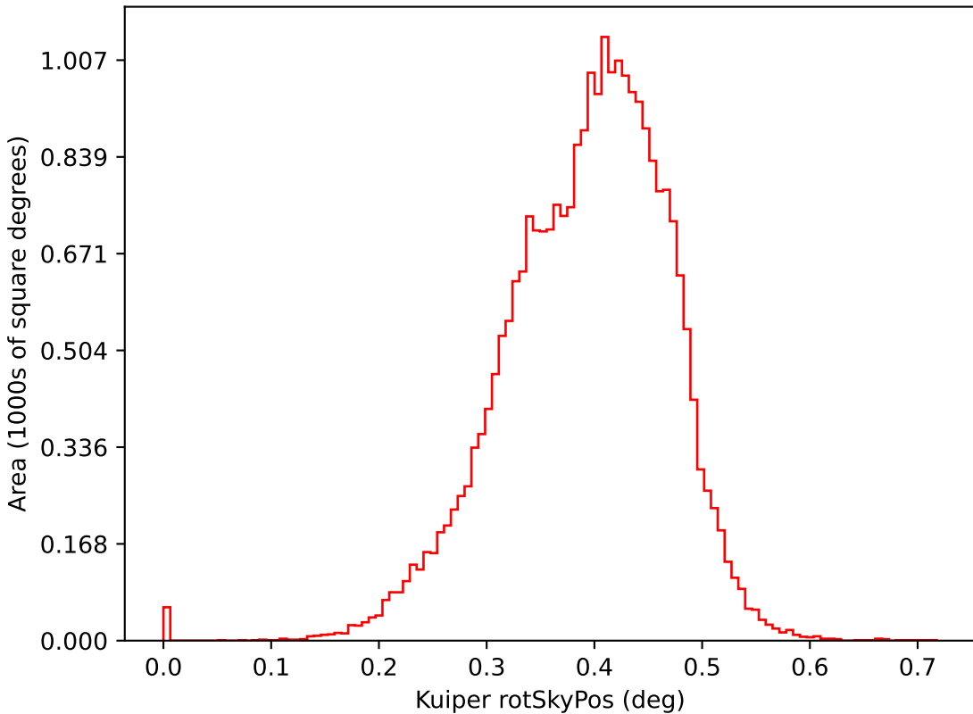
too_elab_r256_d3_giz_v3.4_10yrs i: Kuiper rotSkyPos
