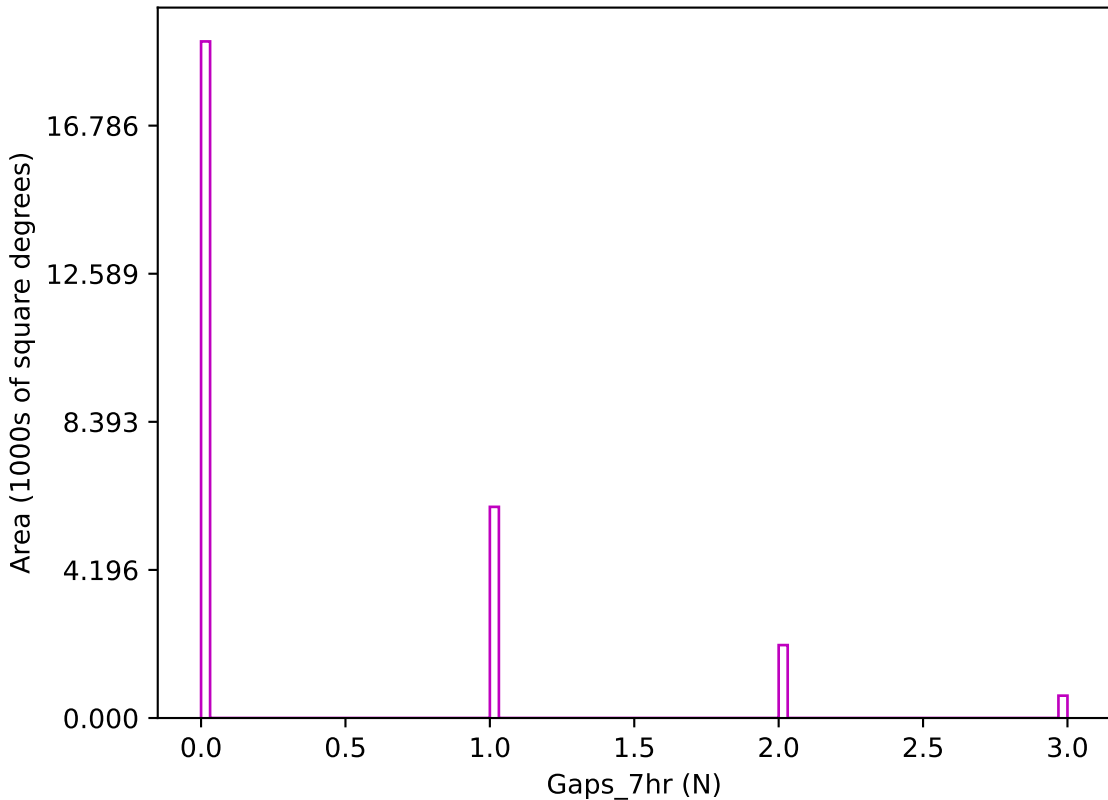
too_elab_r256_d3_giz_v3.4_10yrs z band: Gaps_7hr
