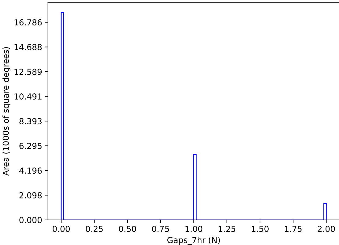
too_elab_r256_d3_giz_v3.4_10yrs y band: Gaps_7hr
