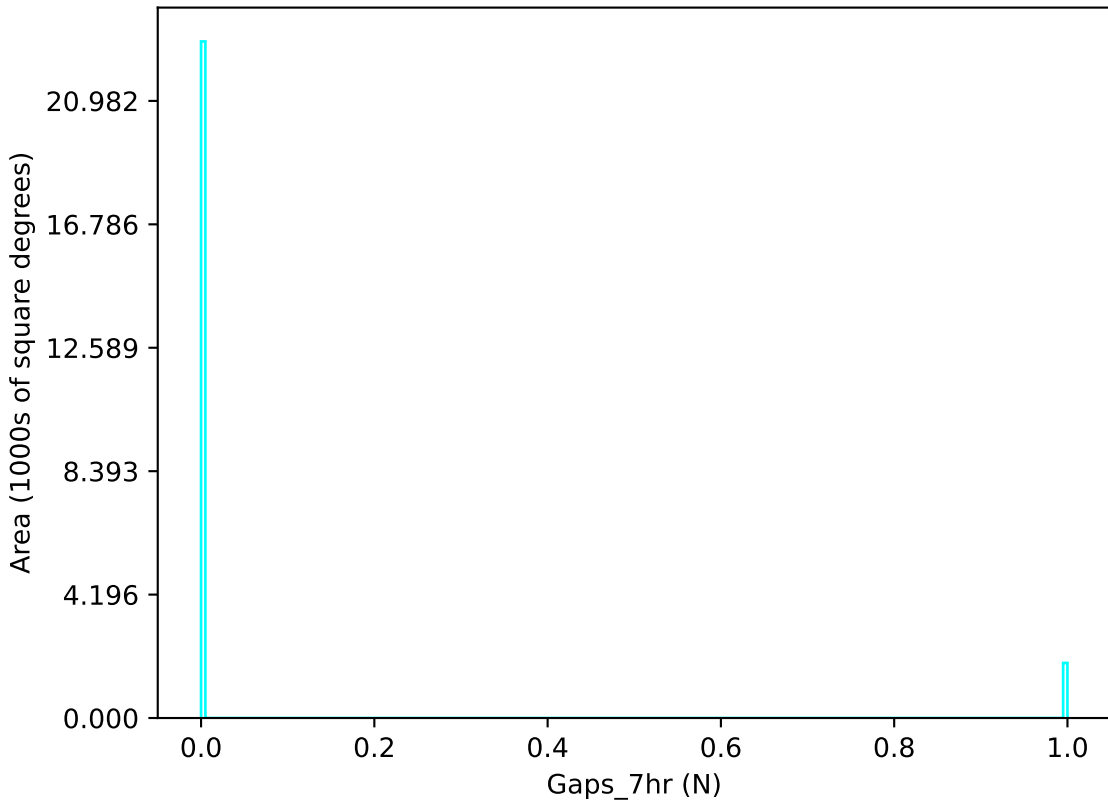
too_elab_r256_d3_giz_v3.4_10yrs u band: Gaps_7hr
