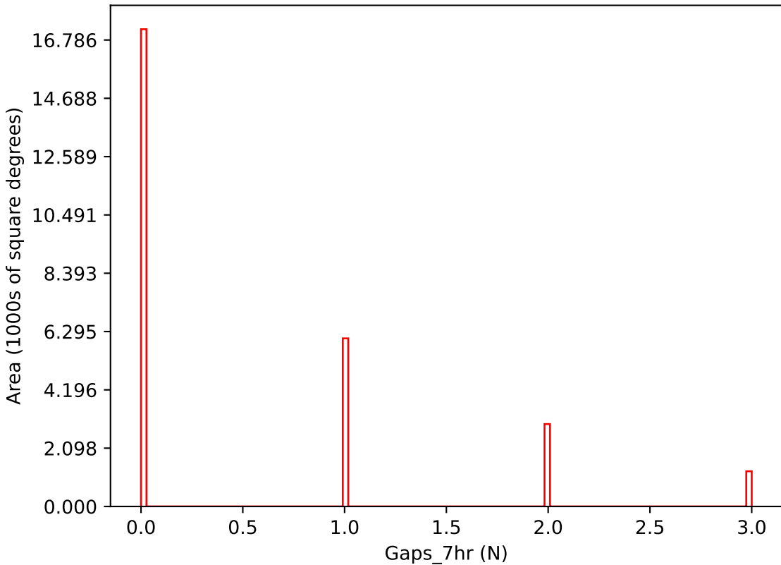
too_elab_r256_d3_giz_v3.4_10yrs i band: Gaps_7hr
