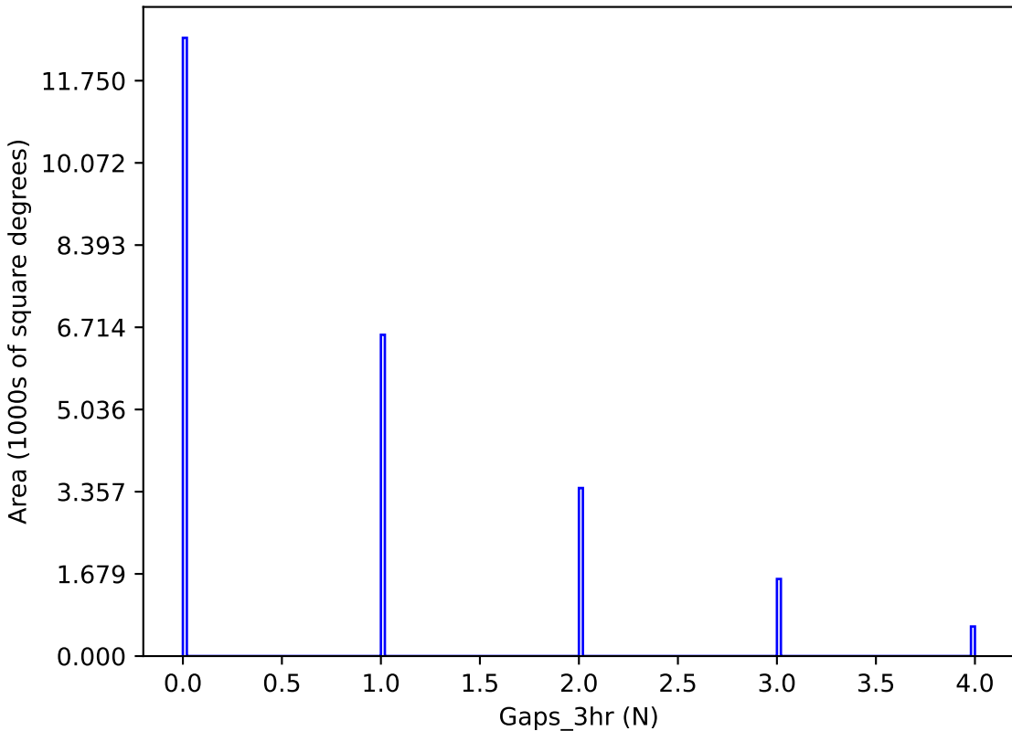
too_elab_r256_d3_giz_v3.4_10yrs y band: Gaps_3hr
