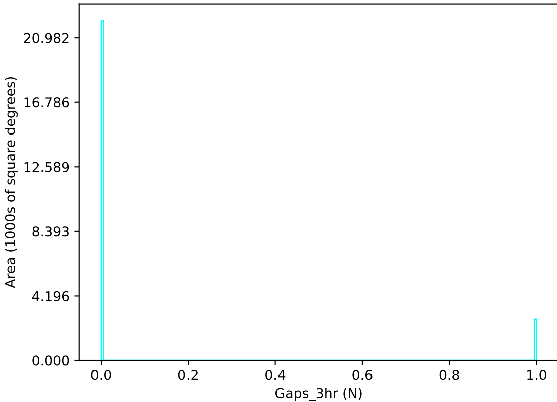
too_elab_r256_d3_giz_v3.4_10yrs u band: Gaps_3hr
