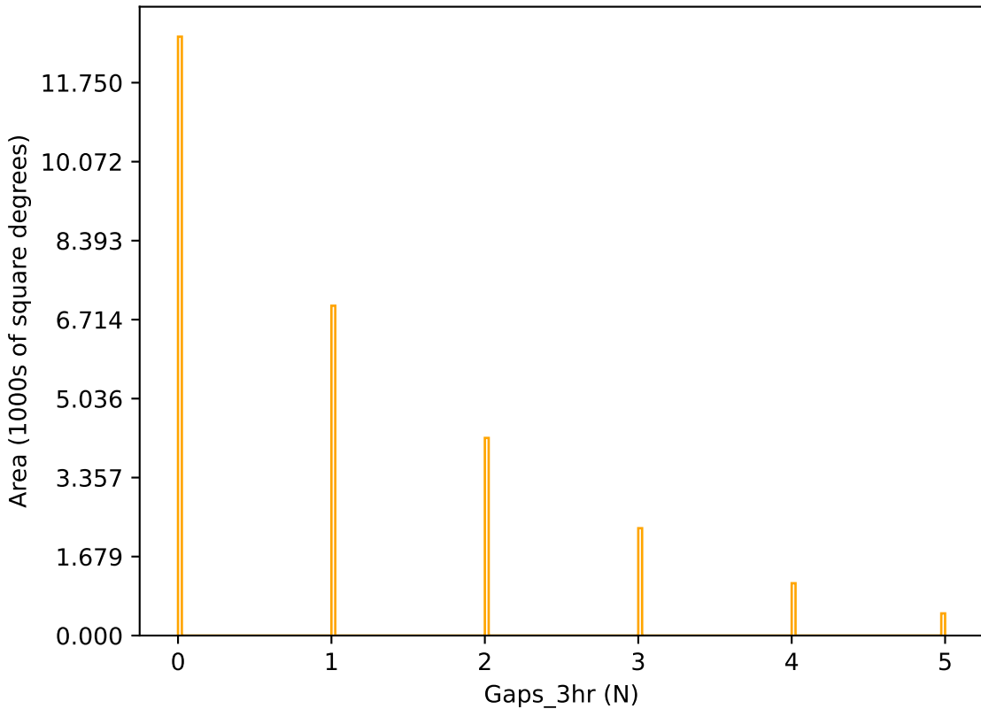
too_elab_r256_d3_giz_v3.4_10yrs r band: Gaps_3hr
