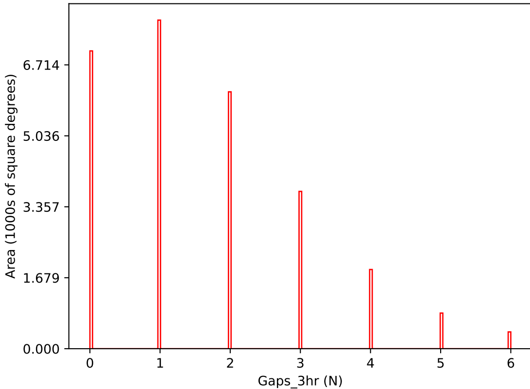
too_elab_r256_d3_giz_v3.4_10yrs i band: Gaps_3hr
