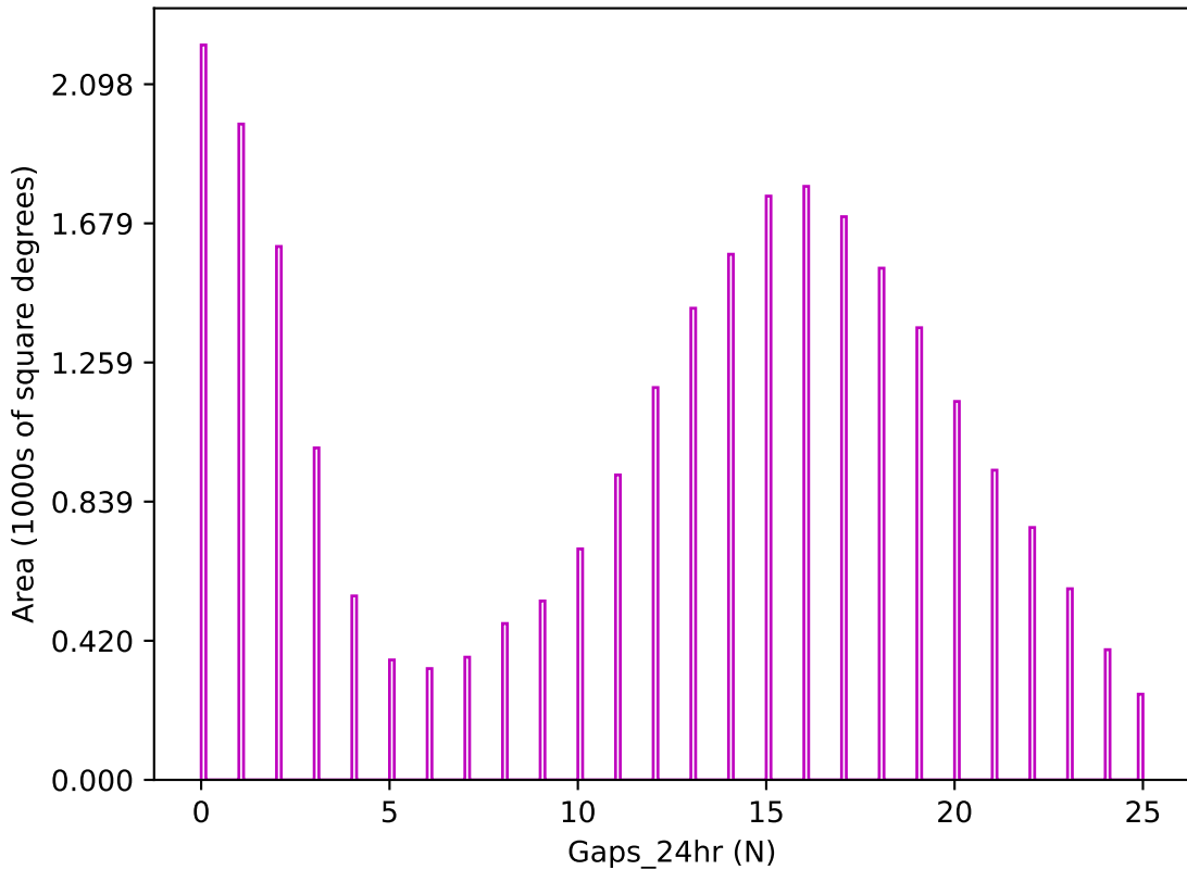
too_elab_r256_d3_giz_v3.4_10yrs z band: Gaps_24hr
