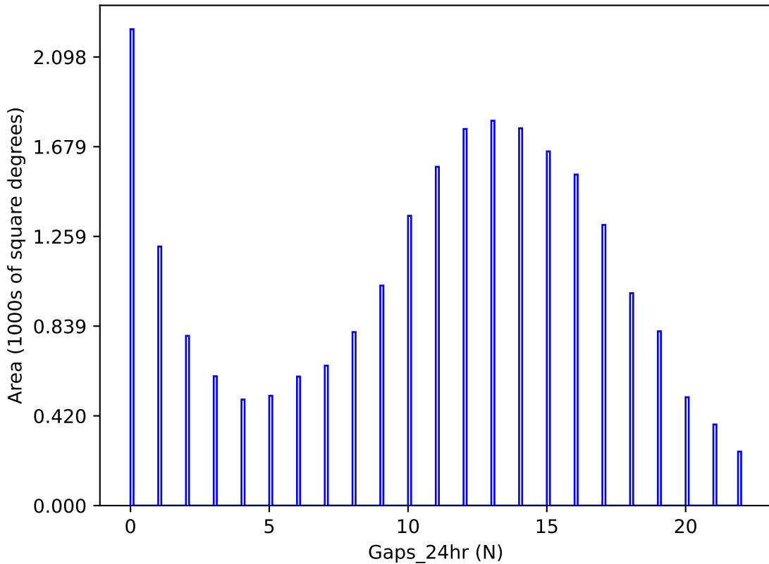
too_elab_r256_d3_giz_v3.4_10yrs y band: Gaps_24hr
