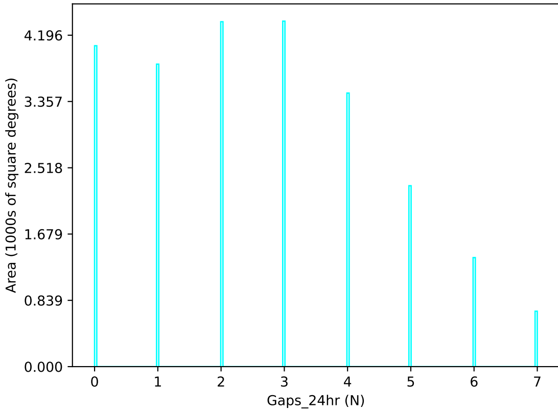
too_elab_r256_d3_giz_v3.4_10yrs u band: Gaps_24hr
