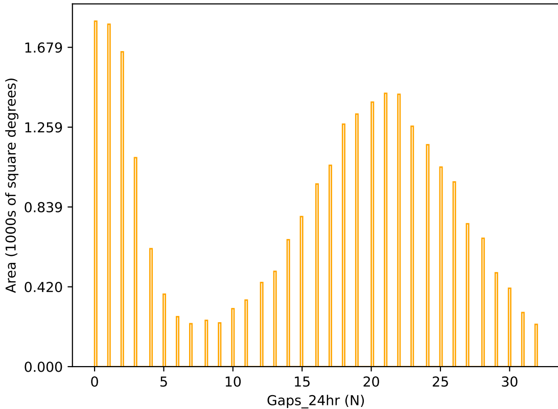
too_elab_r256_d3_giz_v3.4_10yrs r band: Gaps_24hr
