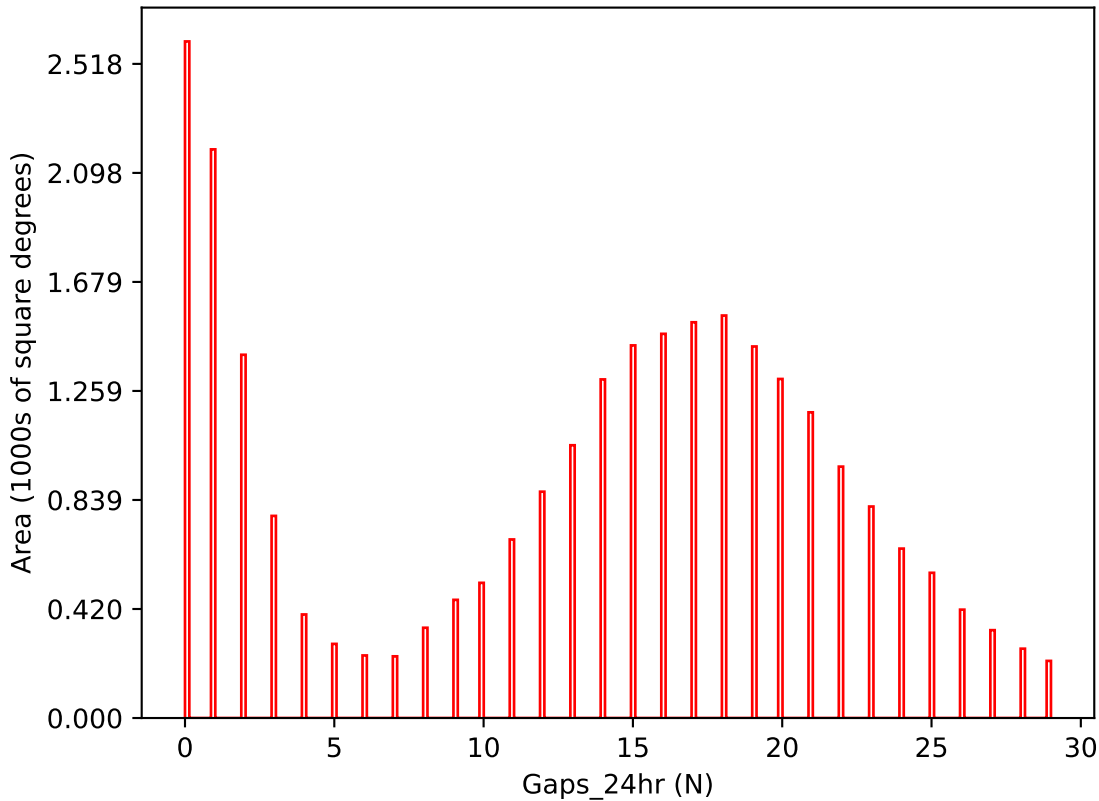
too_elab_r256_d3_giz_v3.4_10yrs i band: Gaps_24hr
