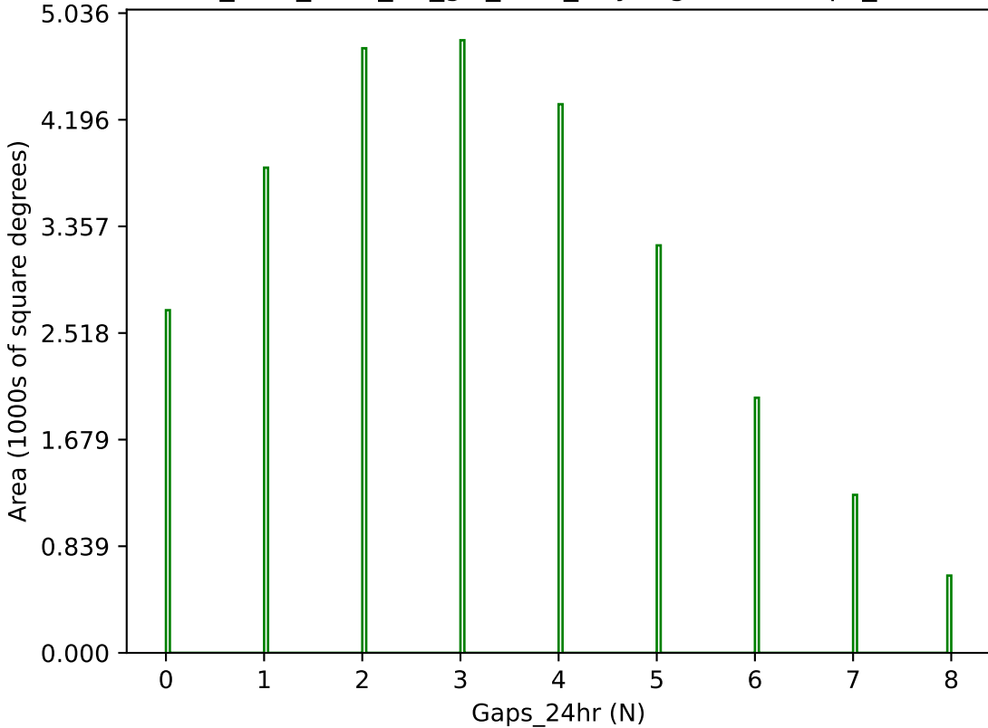
too_elab_r256_d3_giz_v3.4_10yrs g band: Gaps_24hr
