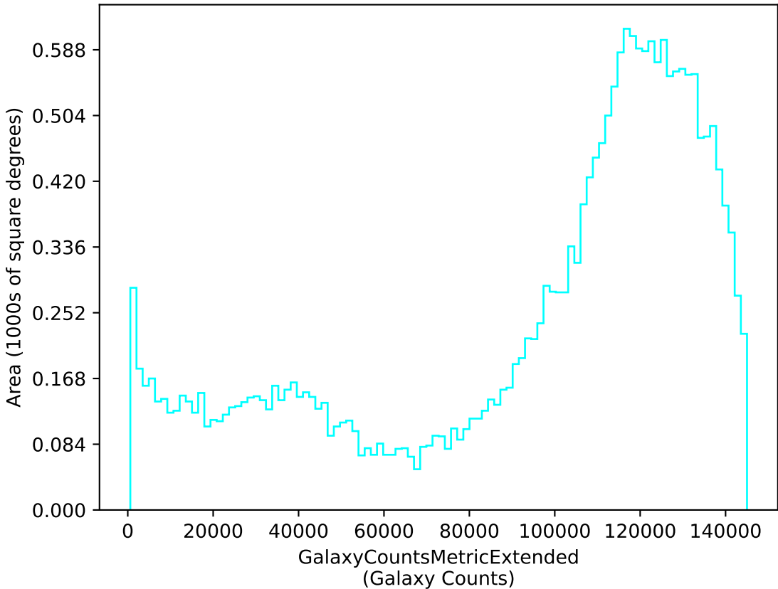
too_elab_r256_d3_giz_v3.4_10yrs u: GalaxyCountsMetricExtended
