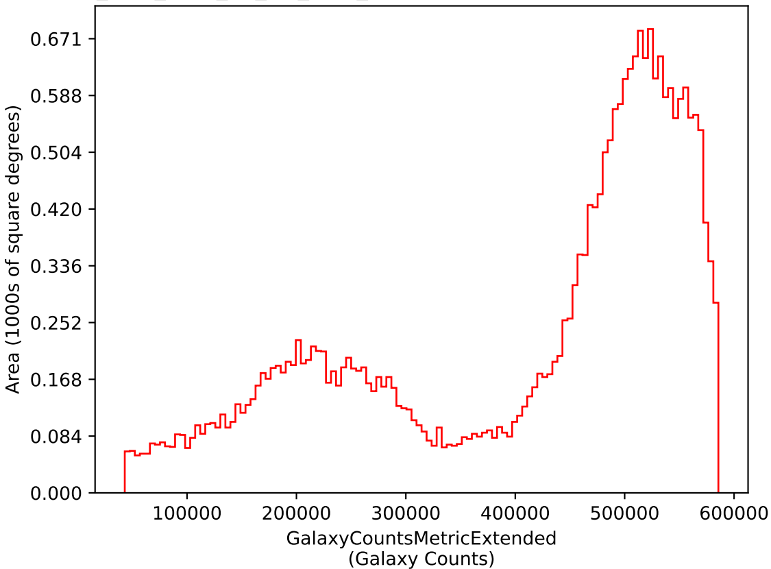
too_elab_r256_d3_giz_v3.4_10yrs i: GalaxyCountsMetricExtended
