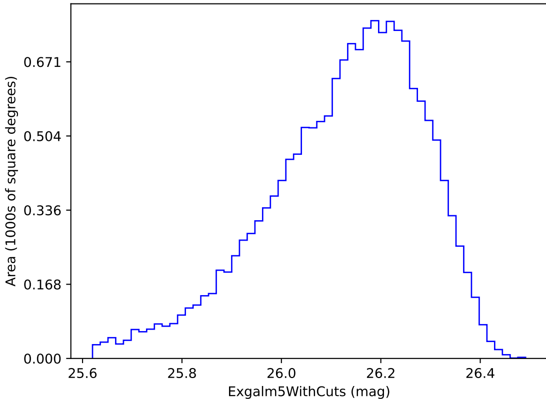
too_elab_r256_d3_giz_v3.4_10yrs i band non-DD year 6: Exgal5WithCuts
