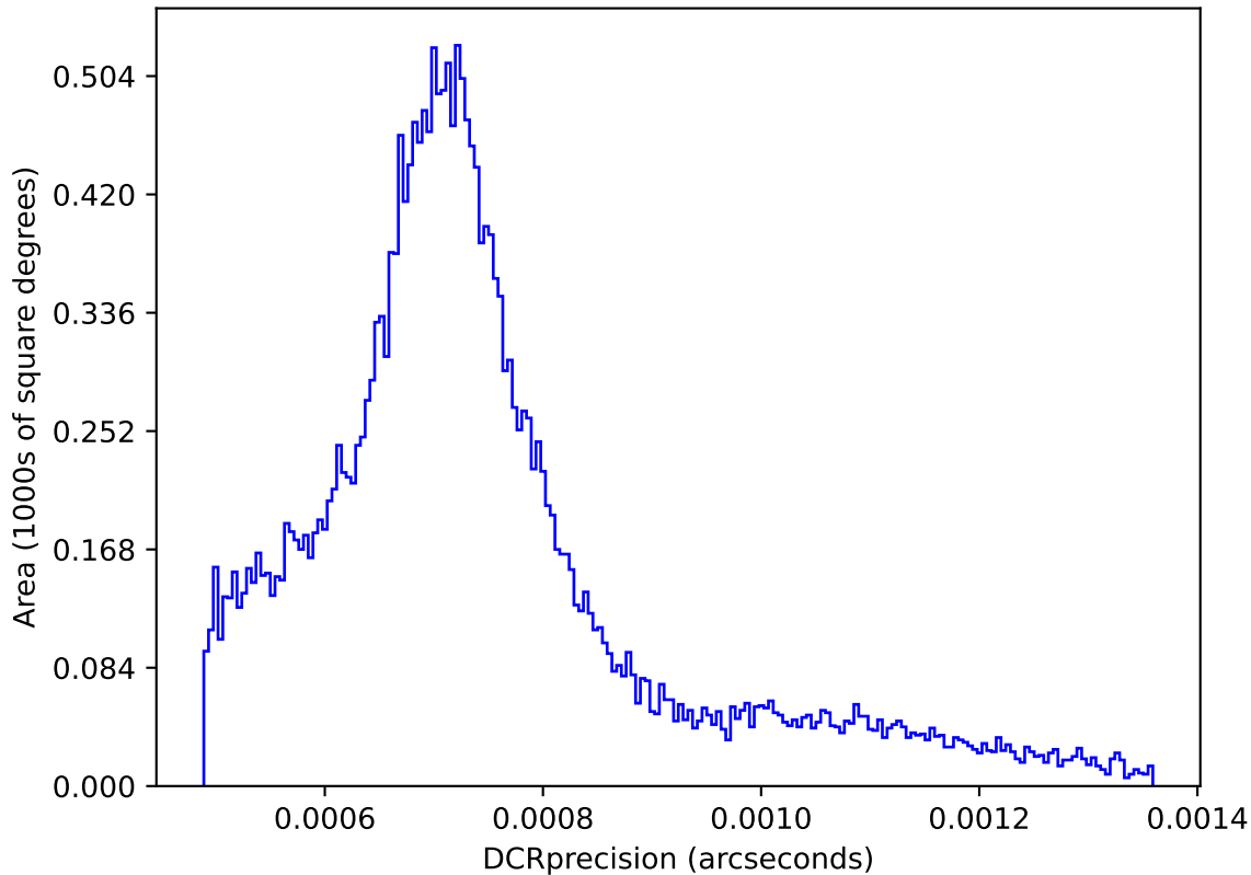
too_elab_r256_d3_giz_v3.4_10yrs : DCRprecision
