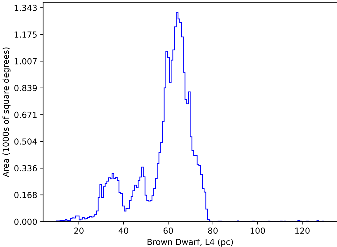
too_elab_r256_d3_giz_v3.4_10yrs : Brown Dwarf, L4
