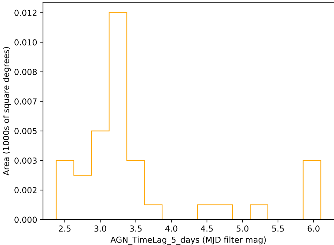
too_elab_r256_d3_giz_v3.4_10yrs r band: AGN_TimeLag_5_days
