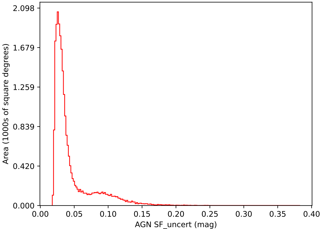
too_elab_r256_d3_giz_v3.4_10yrs i band: AGN SF_uncert
