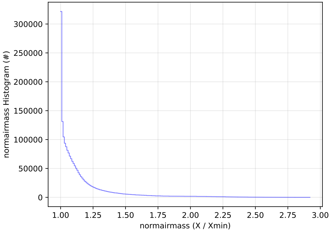
too_elab_r256_d3_giz_v3.4_10yrs WFD all bands: normairmass Histogram
