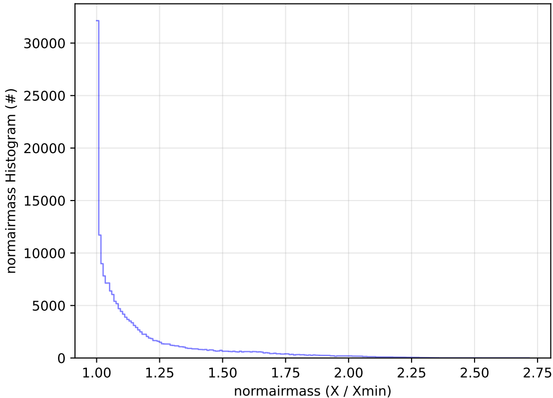
too_elab_r256_d3_giz_v3.4_10yrs All sky g band: normairmass Histogram
