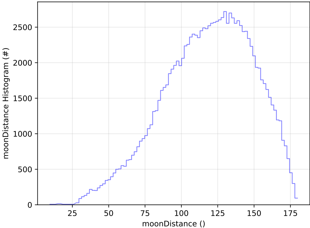
too_elab_r256_d3_giz_v3.4_10yrs All sky u band: moonDistance Histogram
