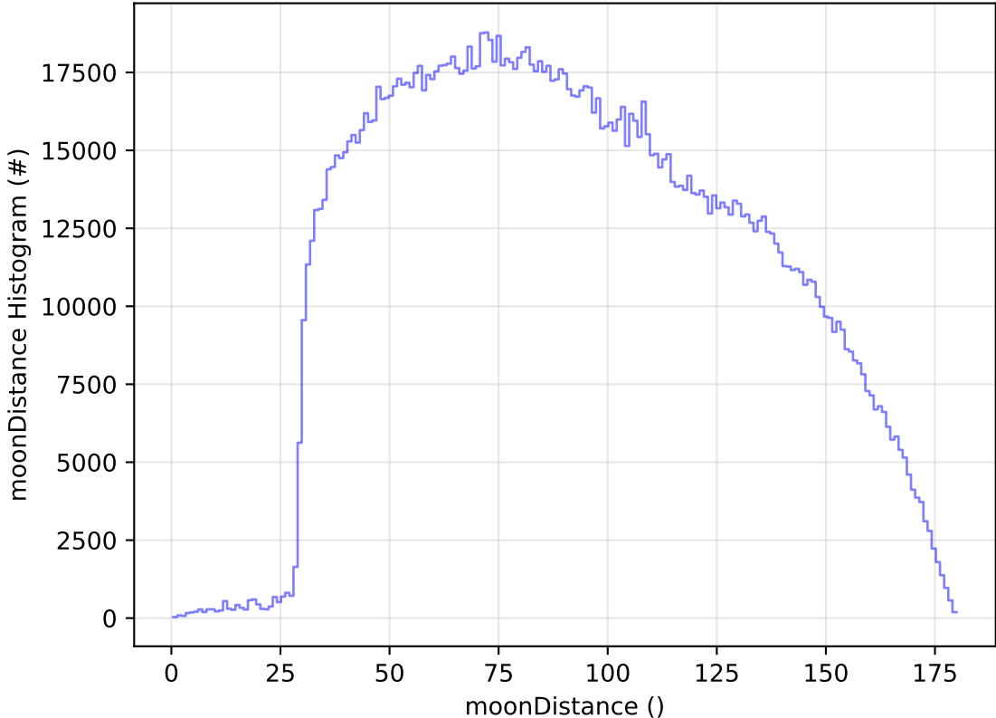
too_elab_r256_d3_giz_v3.4_10yrs All sky all bands: moonDistance Histogram
