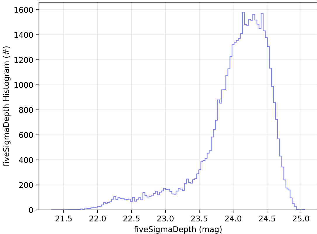
too_elab_r256_d3_giz_v3.4_10yrs Yr 1 r band: fiveSigmaDepth Histogram
