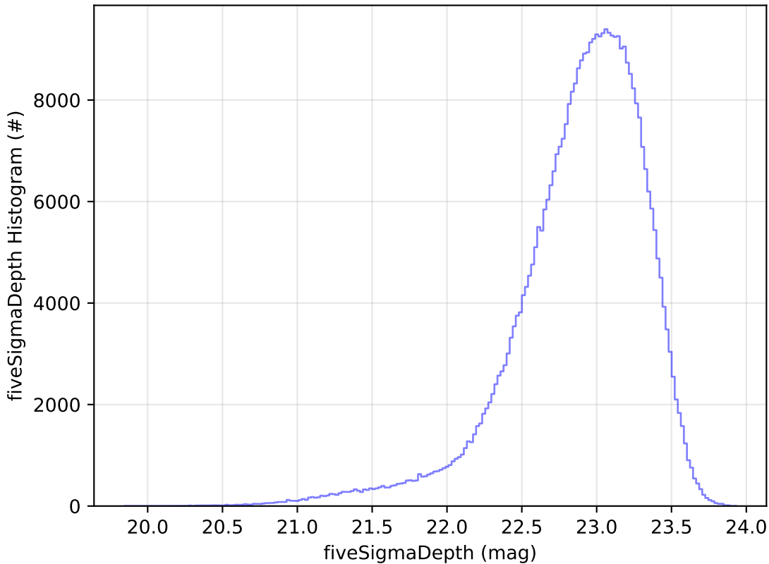
too_elab_r256_d3_giz_v3.4_10yrs WFD z band: fiveSigmaDepth Histogram
