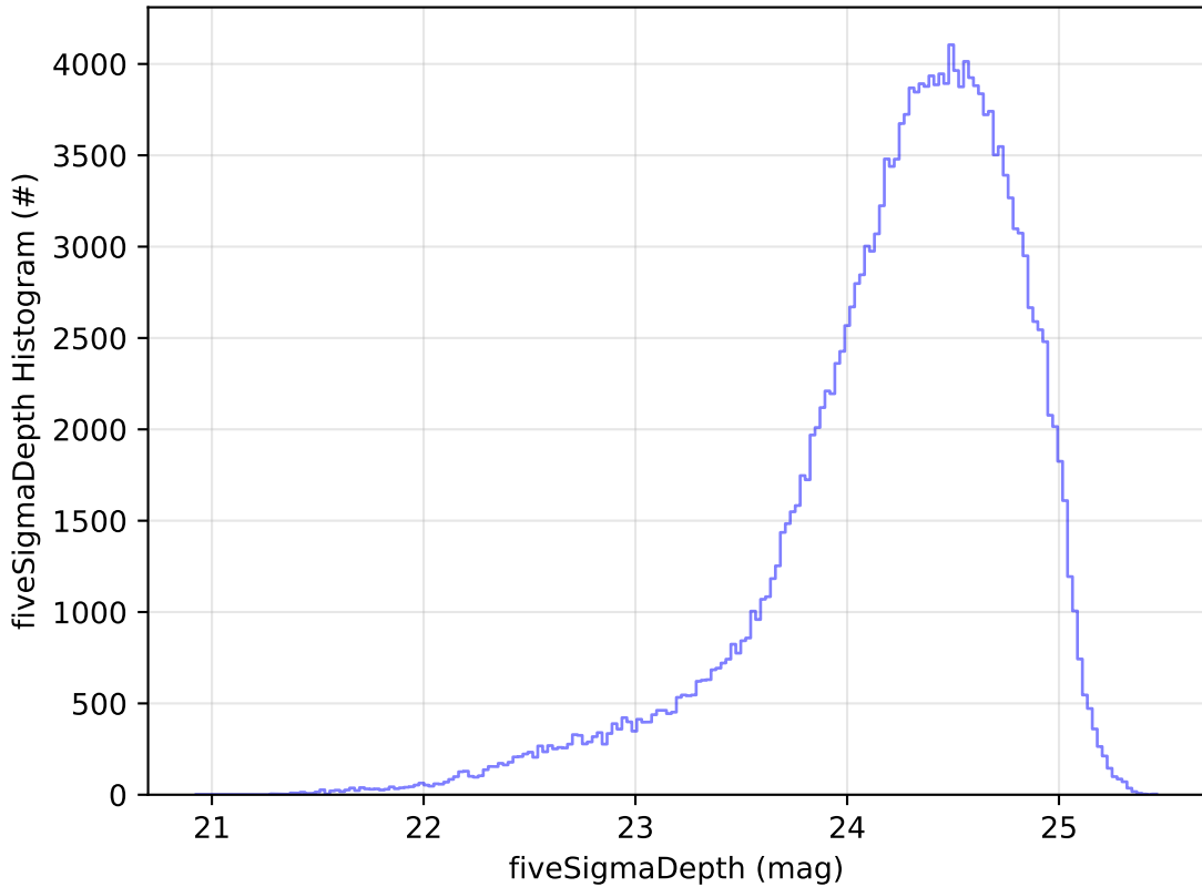
too_elab_r256_d3_giz_v3.4_10yrs All sky g band: fiveSigmaDepth Histogram
