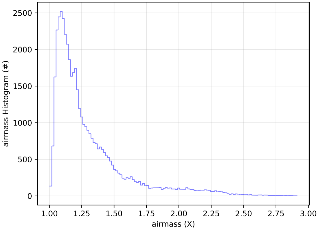
too_elab_r256_d3_giz_v3.4_10yrs Yr 1 z band: airmass Histogram
