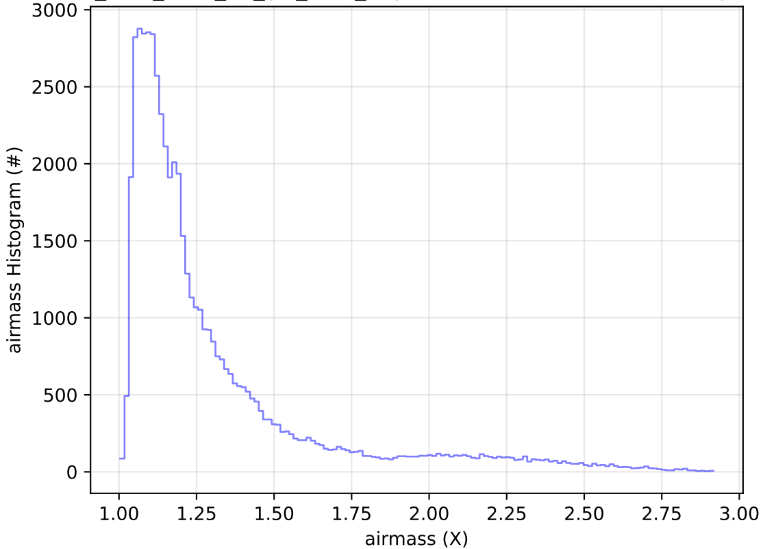
too_elab_r256_d3_giz_v3.4_10yrs Yr 1 i band: airmass Histogram
