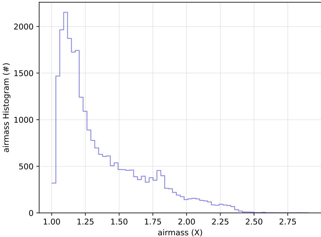
too_elab_r256_d3_giz_v3.4_10yrs Yr 1 g band: airmass Histogram
