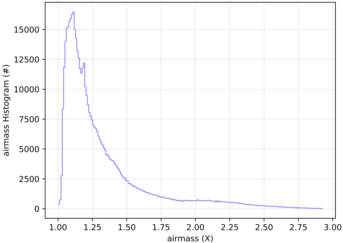
too_elab_r256_d3_giz_v3.4_10yrs WFD i band: airmass Histogram
