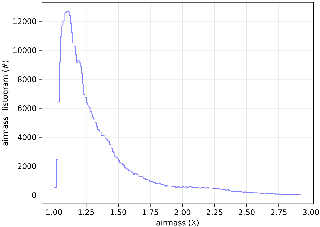
too_elab_r256_d3_giz_v3.4_10yrs All sky z band: airmass Histogram
