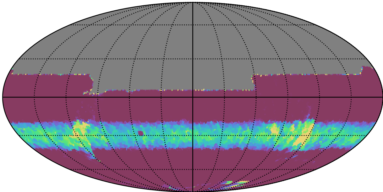
too_elab_r256_d3_giz_v3.4_10yrs All sky y band: Min normairmass
