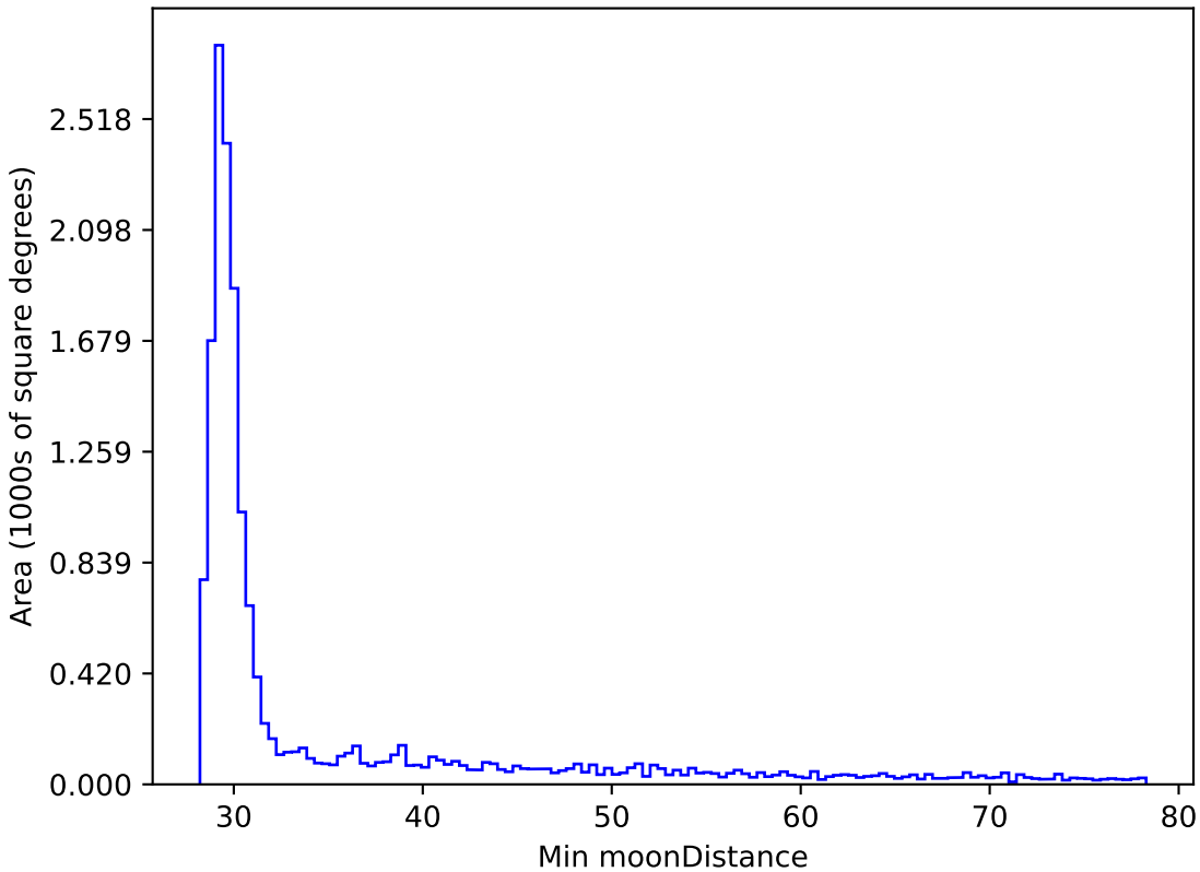
too_elab_r256_d3_giz_v3.4_10yrs WFD y band: Min moonDistance
