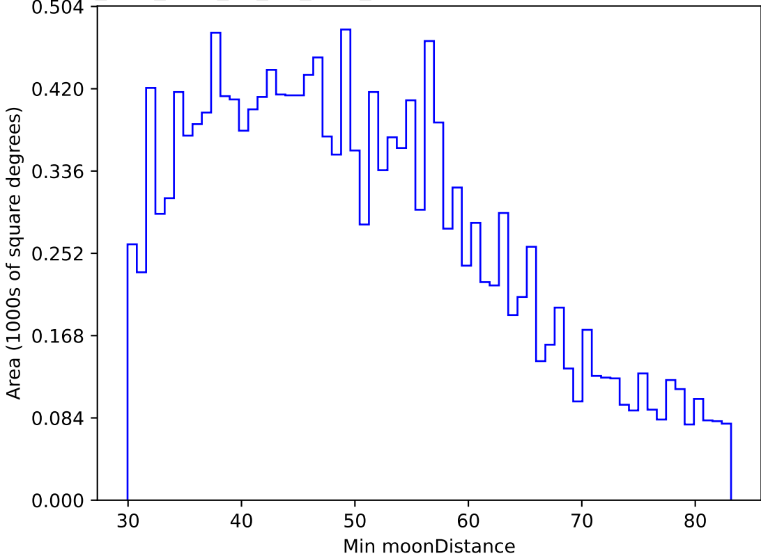
too_elab_r256_d3_giz_v3.4_10yrs WFD u band: Min moonDistance
