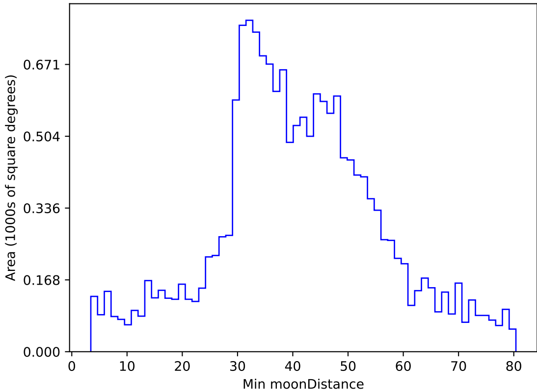
too_elab_r256_d3_giz_v3.4_10yrs WFD g band: Min moonDistance
