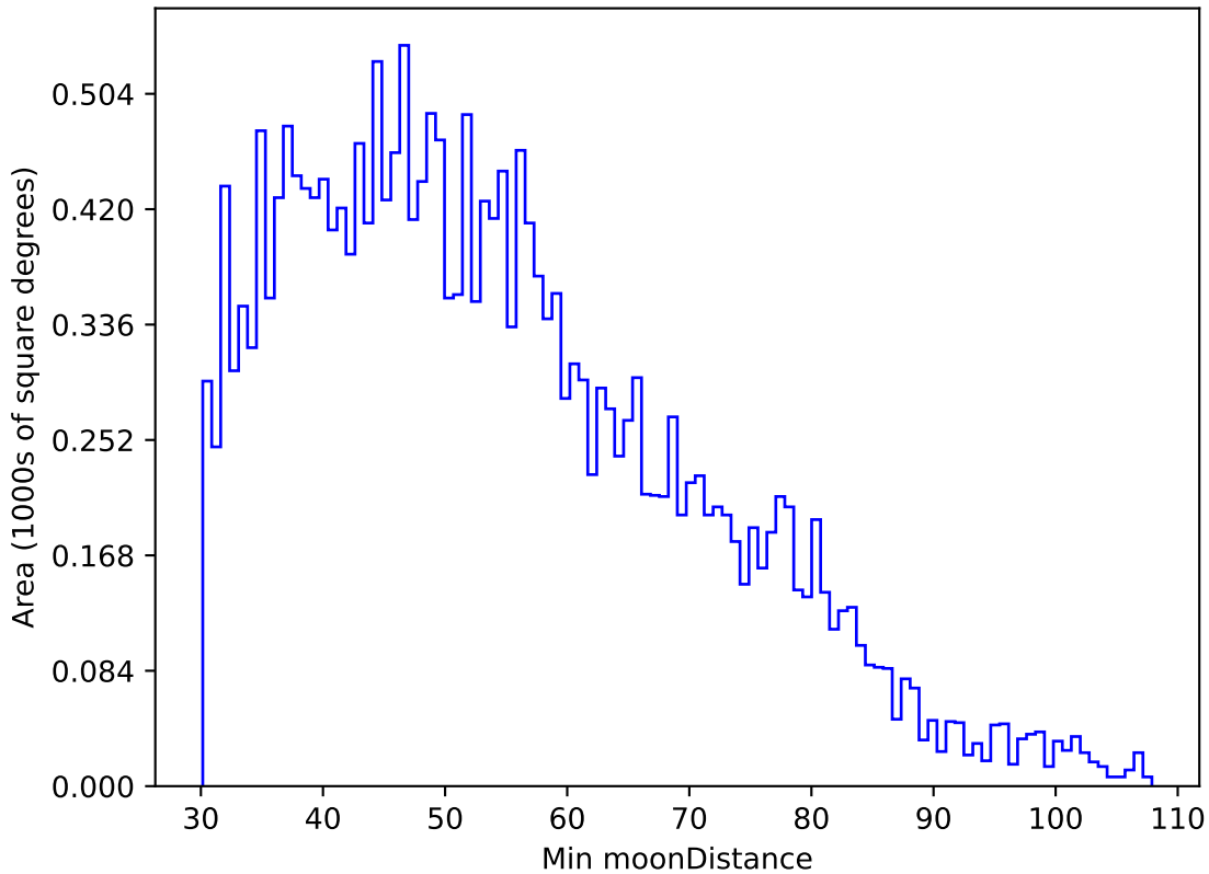
too_elab_r256_d3_giz_v3.4_10yrs All sky u band: Min moonDistance
