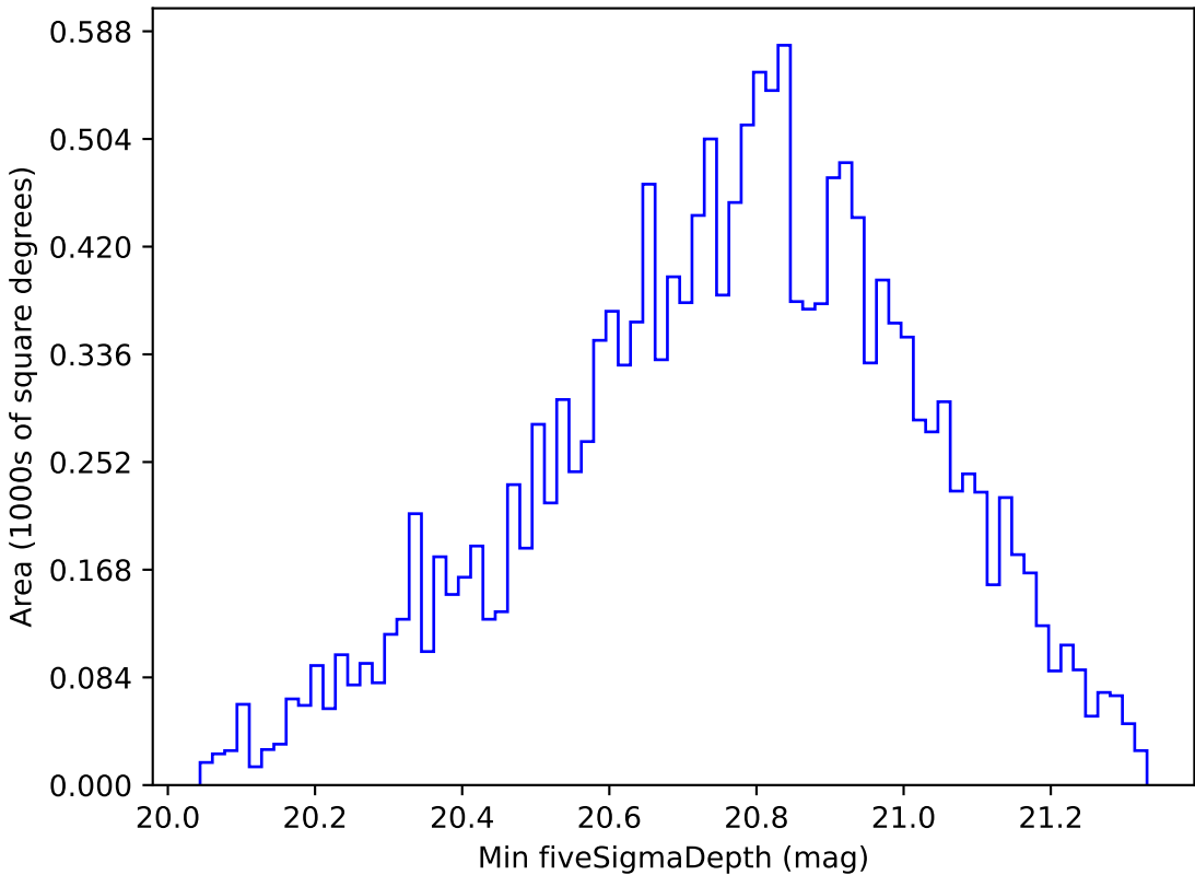
too_elab_r256_d3_giz_v3.4_10yrs WFD all bands: Min fiveSigmaDepth
