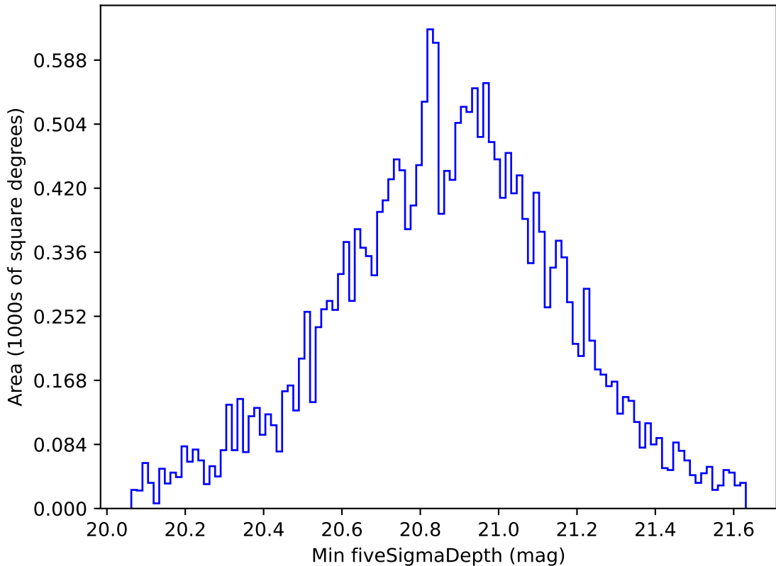
too_elab_r256_d3_giz_v3.4_10yrs All sky y band: Min fiveSigmaDepth
