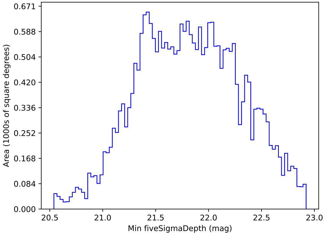
too_elab_r256_d3_giz_v3.4_10yrs All sky i band: Min fiveSigmaDepth
