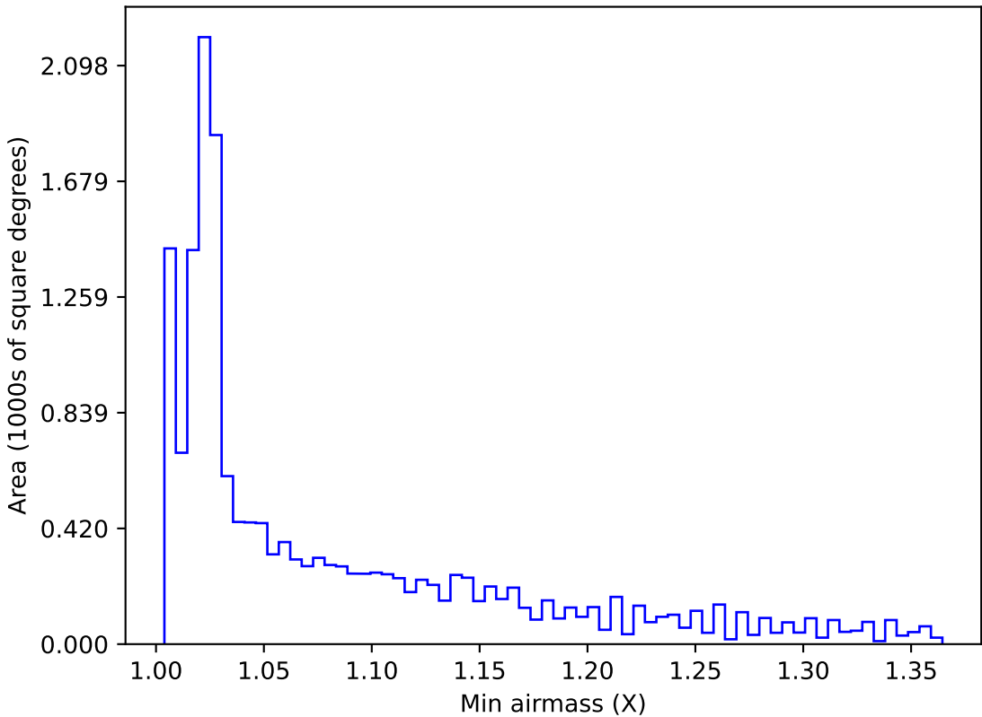
too_elab_r256_d3_giz_v3.4_10yrs WFD all bands: Min airmass
